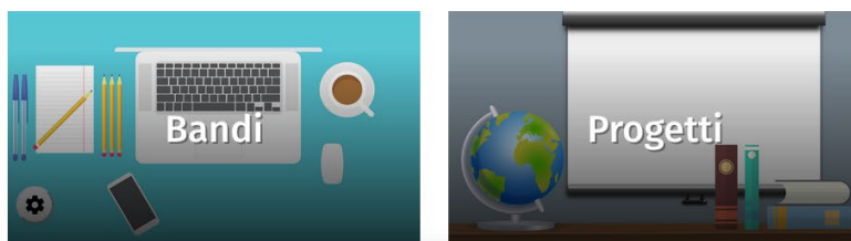
Figura 4 – Dashboard
